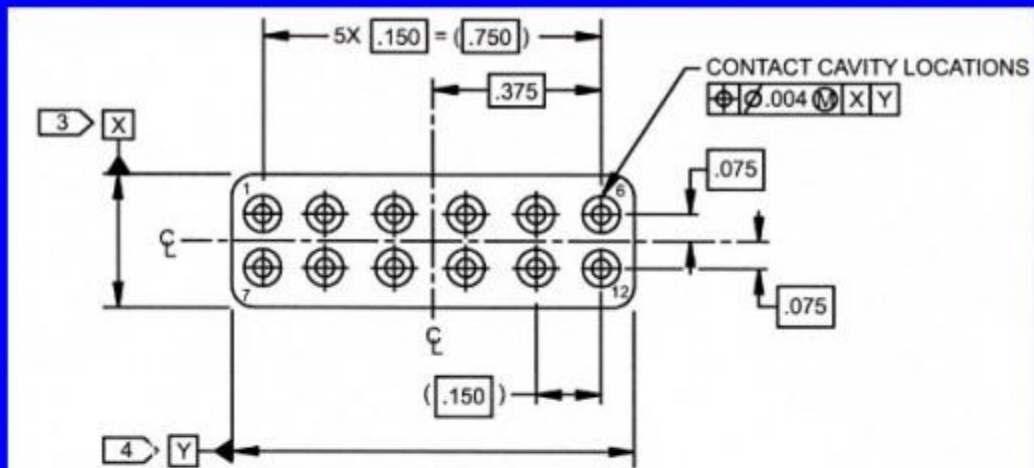
INSERT ARRANGEMENT 4 1 2
